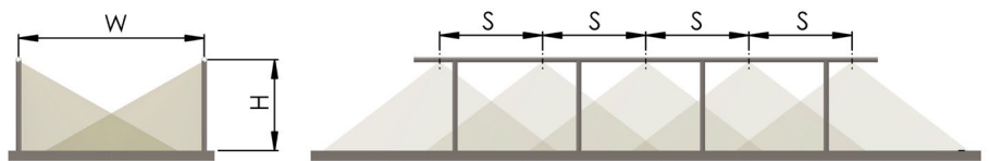
TYPICAL INSTALLATION
